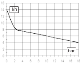
Solenoid ø 100 mm
