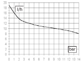
Solenoid ø 110 mm
