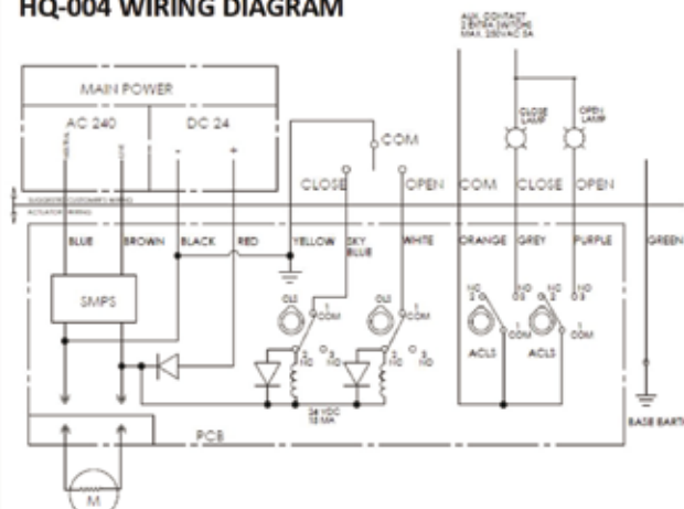
HQ-004 WIRING DIAGRAM
