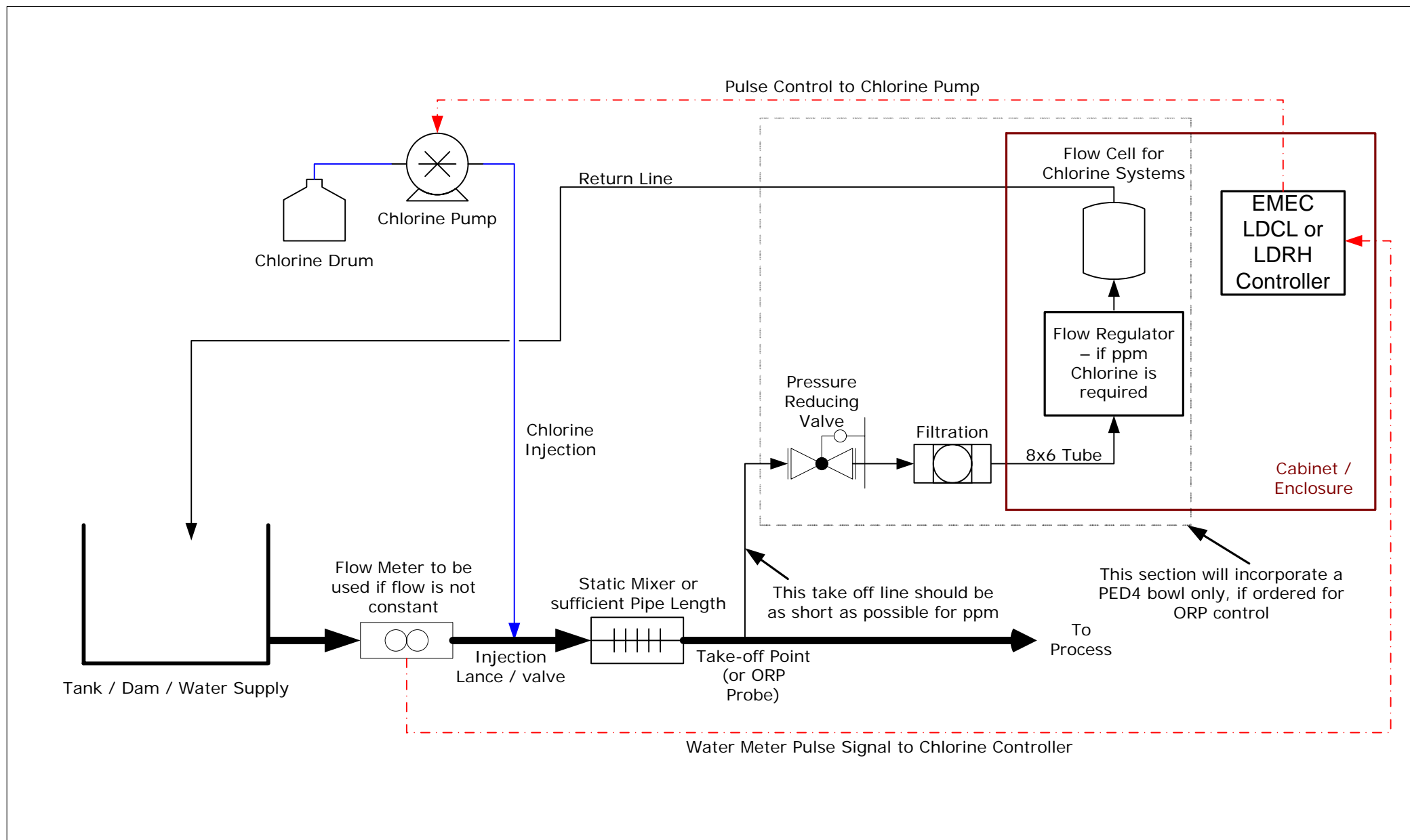
Chlorine Control Set-up Example for In-Line ppm or ORP Control
