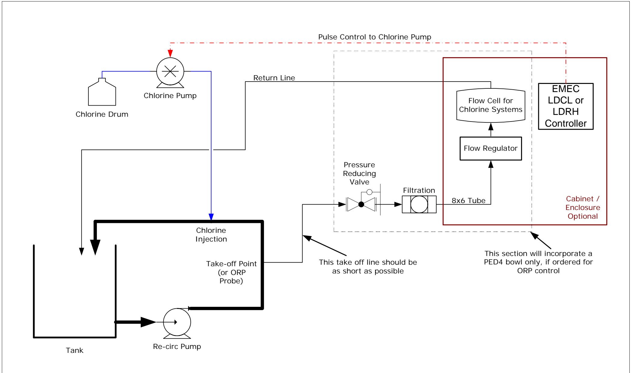
Control Set-up example for Dosing ppm Chlorine into a Re-circulated Tank
