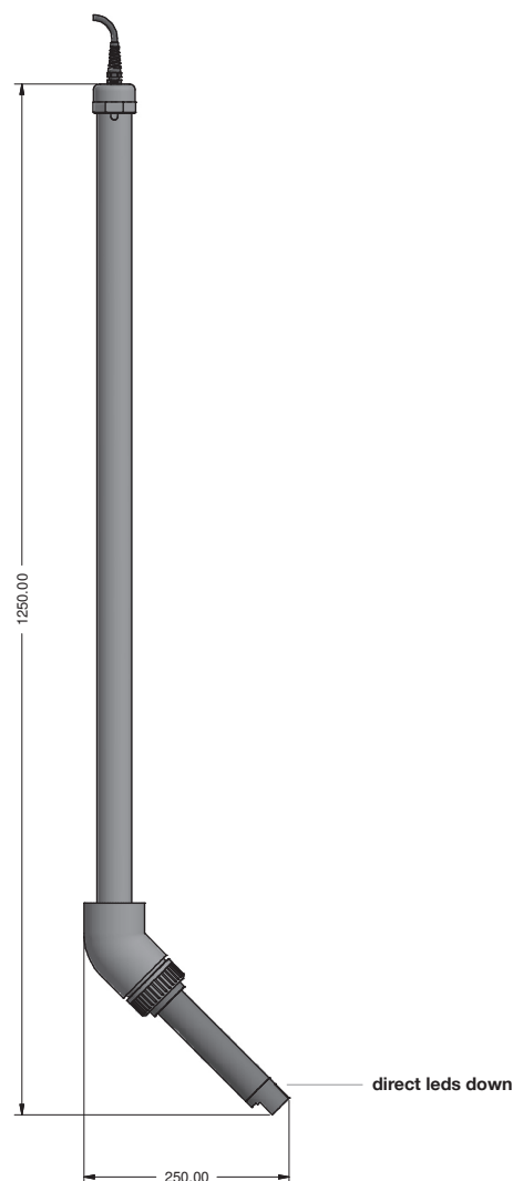
Probe holder for immersion PEC E2
