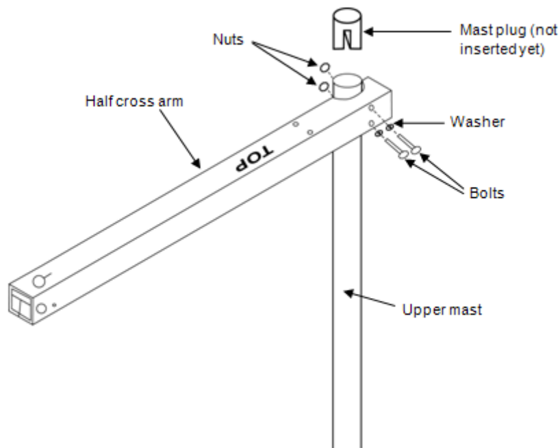
Figure 52: Half cross arm (setup is same for full cross arm)
