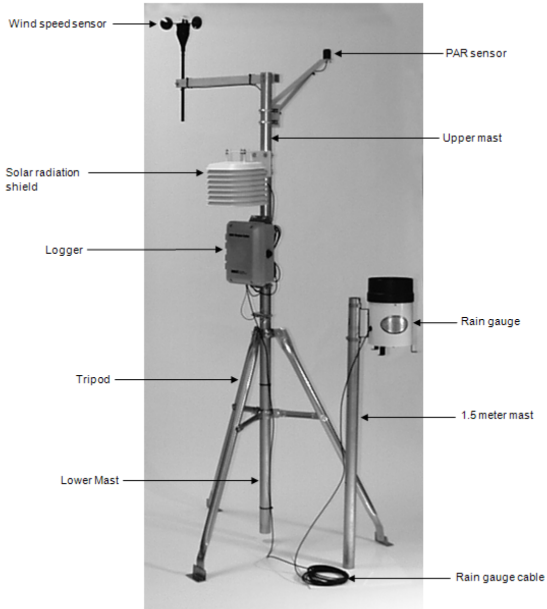
Figure 41: 2 Meter Tri-pod
