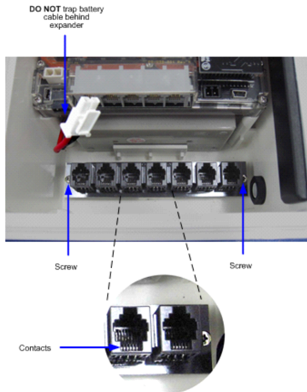
Figure 35: Installing the Expander Board
