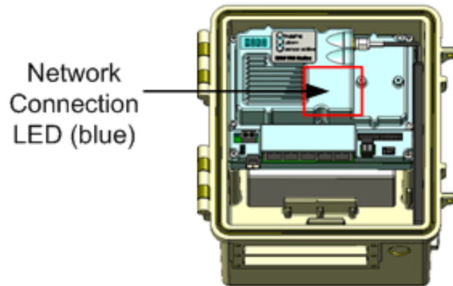
Figure 39: Connection Status LEDs
