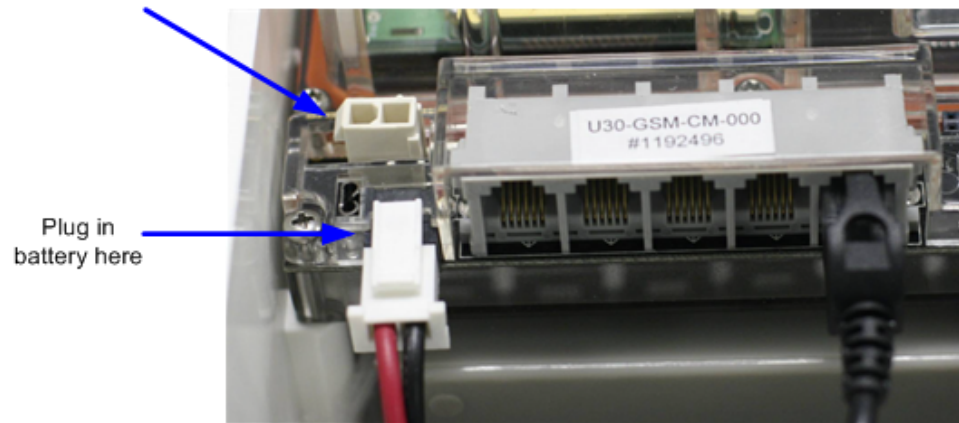
Figure 37: Connecting the Battery
