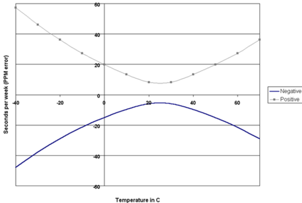
Figure 38: Time Accuracy Graph
