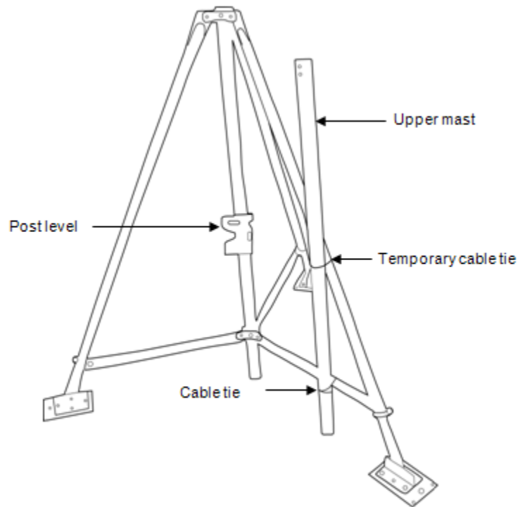
Figure 51: Upper mast (temporary)
