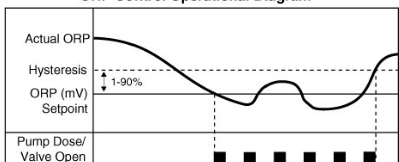
ORP Control Operational Diagram
