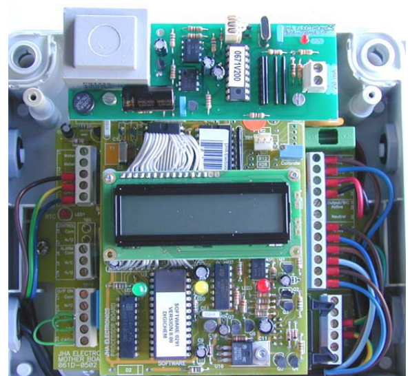
CIRCUIT WITH THE 4-20mA CARD
