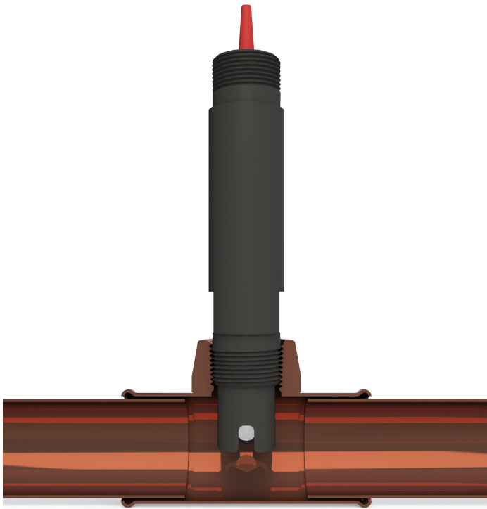
A3: Cross Section of ORP Probe in Manifold
