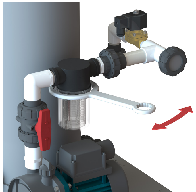
Loosen or Tighten Bowl on RV-ILS 1" or larger Inline Strainers
